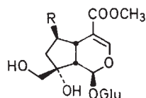
splendoside ( 34 ); R = H 6- \beta -hydroxysplendoside ( 35 ); R = OH
