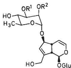
nigroside 1 (91)
