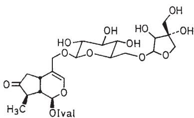
6'-apiosylebuloside ( 38 )
