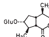
nepetaside (59)
