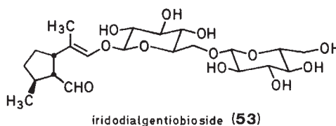
iridodialgentiobioside (53)
