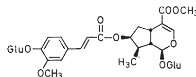
periclymenoside (87)
