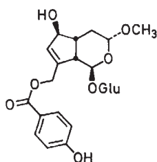
nishindaside (50)
