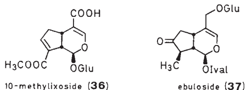
10-methylxoside ( 36 )
