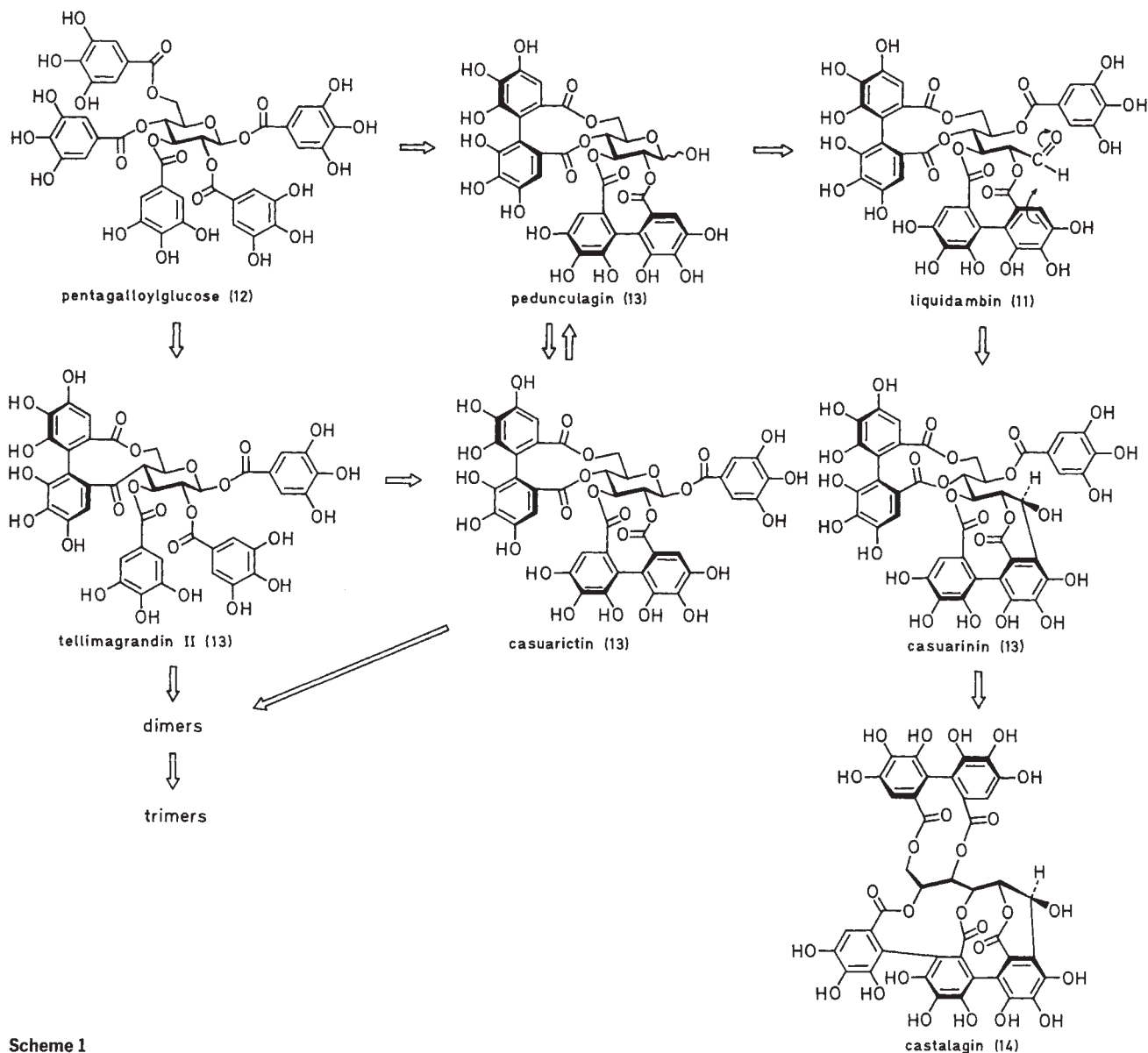
Scheme 1
