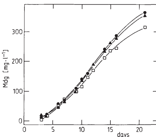
Fig. 3. Biotransformation of \beta -methylidigitoxin (Mdg) in a shake culture of Digitalis lanata (strain 287). Glucose was fed from day 8 to maintain a glucose level of between 2 and 5 g·l -1 . A aliquot of culture medium was diluted with methanol and analysed by HPLC (28).
