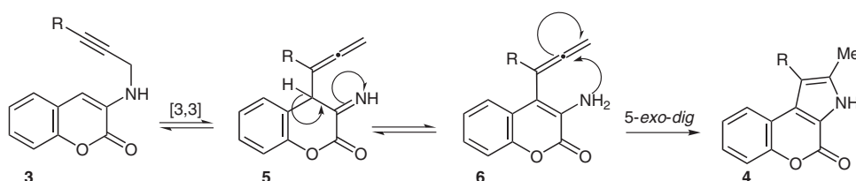
Scheme 3 Probable mechanism of the amino-Claisen rearrangement
