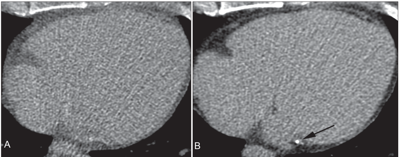
Figure 1 (A-B): The CS raw data image (A) shows no obvious calcification at 55% R-R reconstruction, whereas the calcified plaque (arrow) is well seen in the circumflex artery at 65% reconstruction (B).
