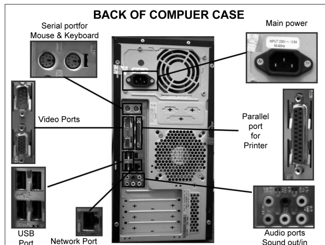
Figure 2: Back of a computer, showing important parts. The input and output devices are interfaced here
