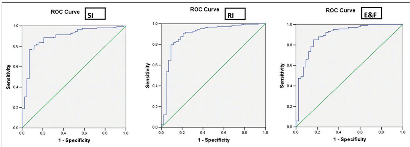
Figure 2: Receiver operator characteristic curves of Srivastava index, Ricerca index and England and Fraser index
