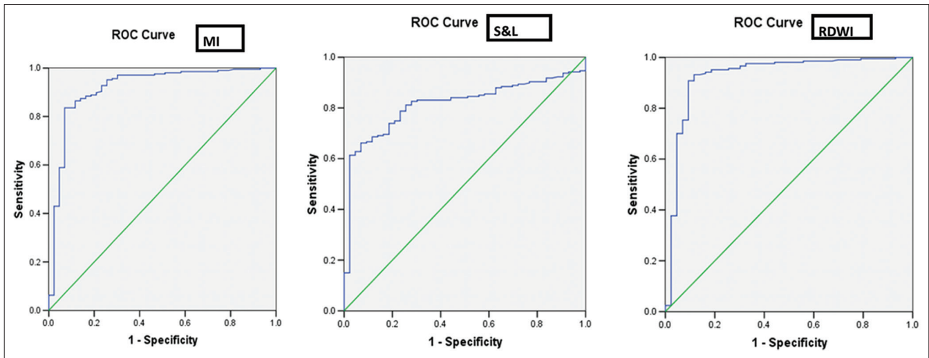
Figure 1: Receiver operator characteristic curves of Mentzer index, Shine and Lal index and red cell distribution width index
