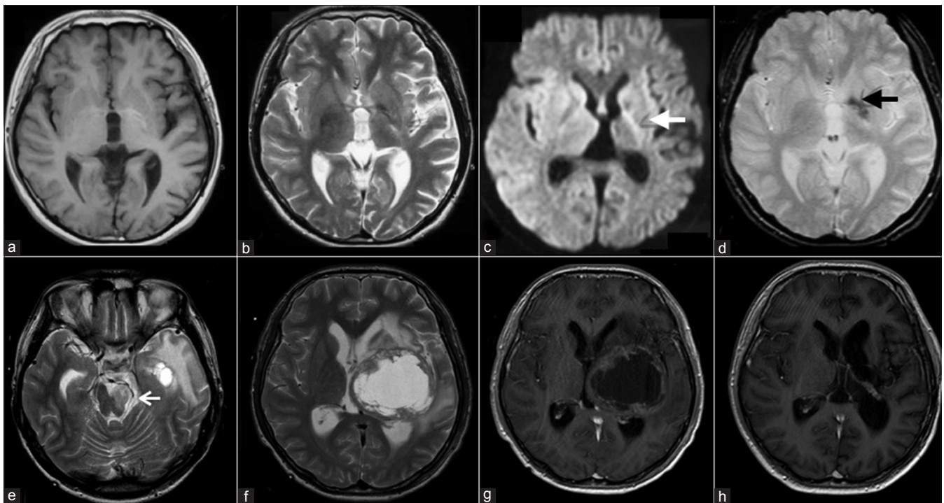
Figure 1: Initial T1W magnetic resonance imaging (MRI): Left hemispheric atrophy with diffuse sulcal widening and prominent left sylvian fissure without ventricular enlargement (a); T2W: Subtle hyperintense signal changes at the left globus pallidus and posterior limb of the internal capsule (b); DWI: Restricted diffusion of the same areas (white arrow, c) and GRE: Hypointense signals (“blooming”) (black arrow, d); 2 years later: Large left basal ganglia cystic lesion (T2W with left cerebral peduncle atrophy, white thin arrow (e); T2W (f); contrast T1W (g); 6-month post-treatment contrast T1W MRI showed no recurrent tumor (h)
