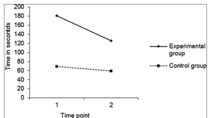
Figure 2: Bigger and more significant changes in time for the experimental group ( \Delta Me = 55 ; \Delta Mk = 9, 75 ) compared with the control group
