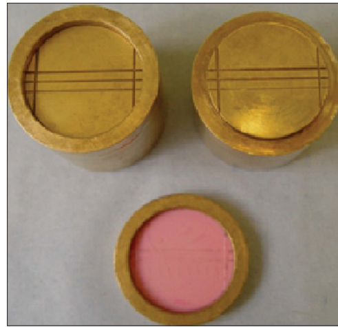
Figure 1: Stainless steel test die constructed according to American dental association specification no: 18 for alginate impression material
