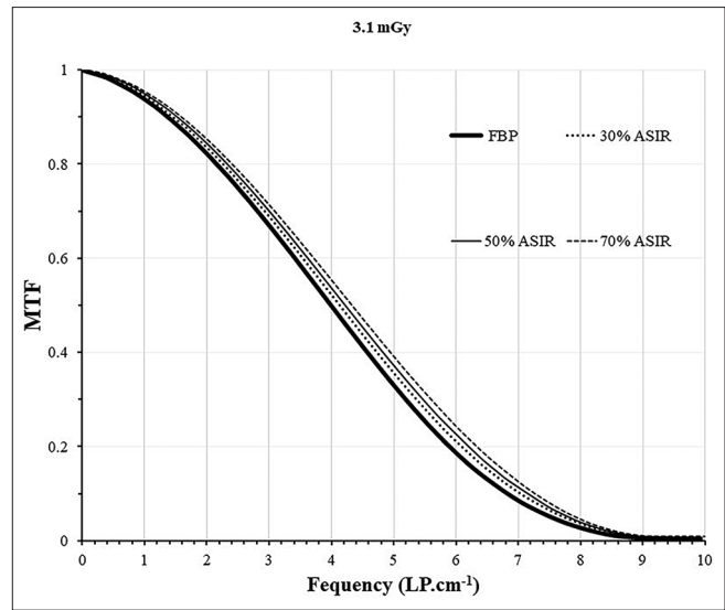
Figure 5: Variation of spatial resolution with different reconstruction methods for the recommendation protocol of 3.1 mGy
