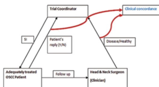
Figure 1: Study algorithm
