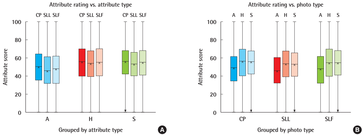
Fig. 3. Marginal mean score of various treatments
